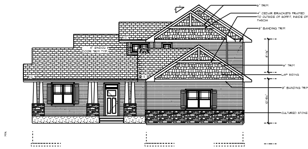
FRONT ELEVATION 1/8" = 1'-0"
