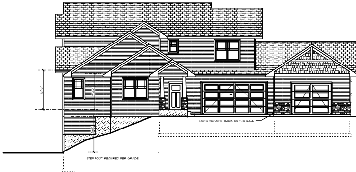
LEFT ELEVATION 1/8" = 1'-0"
