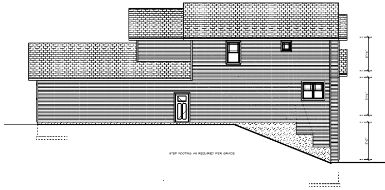
RIGHT ELEVATION 1/8" = 1'-0"
